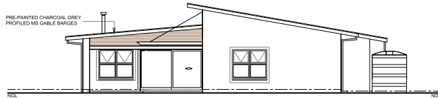
SOUTH EAST ELEVATION
