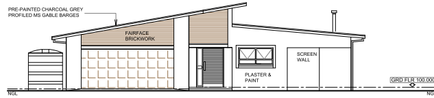
NORTH WEST ELEVATION
